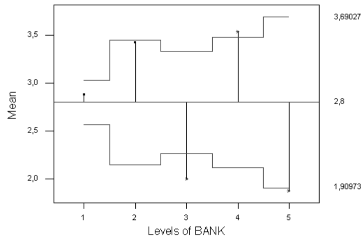
Figure 3. An example of one-way ANOM chart
